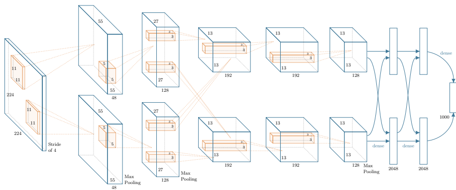
Figure 21: AlexNet architecture.
