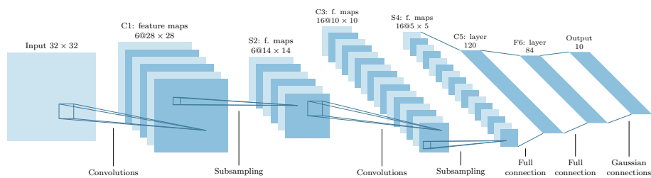
Figure 20: LeNet architecture.
