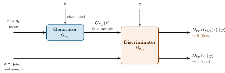
Figure 46: The cGAN architecture: identical to the base GAN in Figure 45, except that both the generator and the discriminator are additionally conditioned on a label y .
