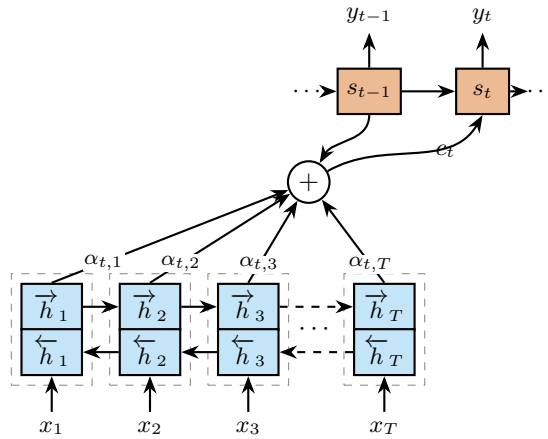
Figure 36: RNN with attention: a bidirectional encoder produces hidden states \mathbf{h}_j ; alignment weights \alpha_{t,j} combine them into the context vector \mathbf{c}_t that feeds the decoder state \mathbf{s}_t generating y_t .
