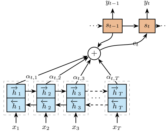
Figure 36: RNN with attention: a bidirectional encoder produces hidden states \vec{h}_j ; alignment weights \alpha_{t,j} combine them into the context vector \mathbf{c}_t that feeds the decoder state \mathbf{s}_t generating y_t .
