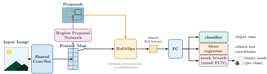
Figure 29: The Mask R-CNN architecture: it extends Faster R-CNN by replacing RoI Pooling with RoIAlign, which uses bilinear interpolation instead of quantization to preserve precise spatial alignment, and by adding a third sibling head, the mask branch, that predicts a binary mask for each RoI alongside the classifier and bounding box regressor.
