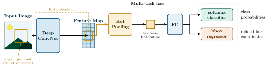
Figure 27: The Fast R-CNN architecture: the whole image is passed once through a deep ConvNet to produce a shared feature map. Each region proposal is projected onto this feature map and reshaped by the RoI pooling layer into a fixed-size feature vector, which is then fed to fully connected layers ending in a softmax classifier and a bounding box regressor, jointly optimized with a multi-task loss.
