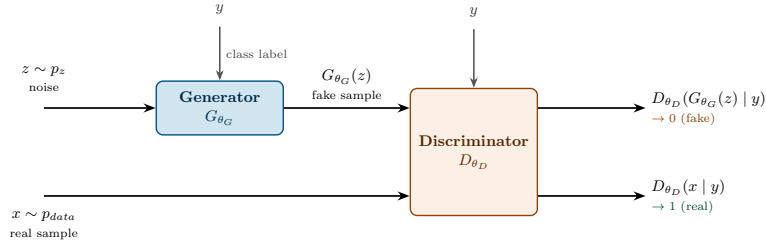
Figure 42: The cGAN architecture: identical to the base GAN in Figure 41, except that both the generator and the discriminator are additionally conditioned on a label y .
