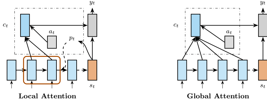
Figure 38: Local vs global attention. Global attention scores all encoder states \mathbf{h}_i at every step, whereas local attention restricts the context to a window centered on the predicted position p_t .
