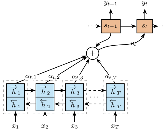
Figure 36: RNN with attention: a bidirectional encoder produces hidden states \mathbf{h}_j ; alignment weights \alpha_{t,j} combine them into the context vector \mathbf{c}_t that feeds the decoder state \mathbf{s}_t generating y_t .
