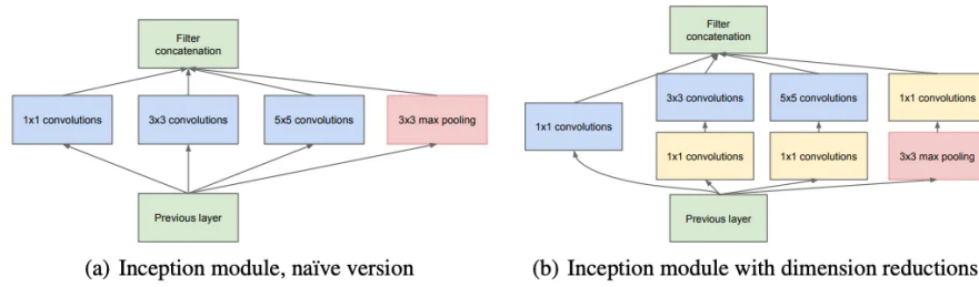
Figure 24: Inception Module.
