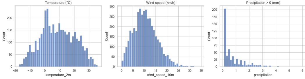
Figure 8: Temperature, wind speed and precipitation distributions over time.
