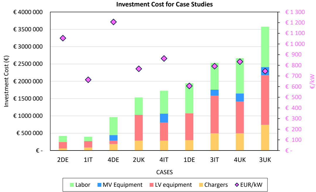
Figure 7: Investment cost and specific cost (€/kW) for the nine public parking case studies.
