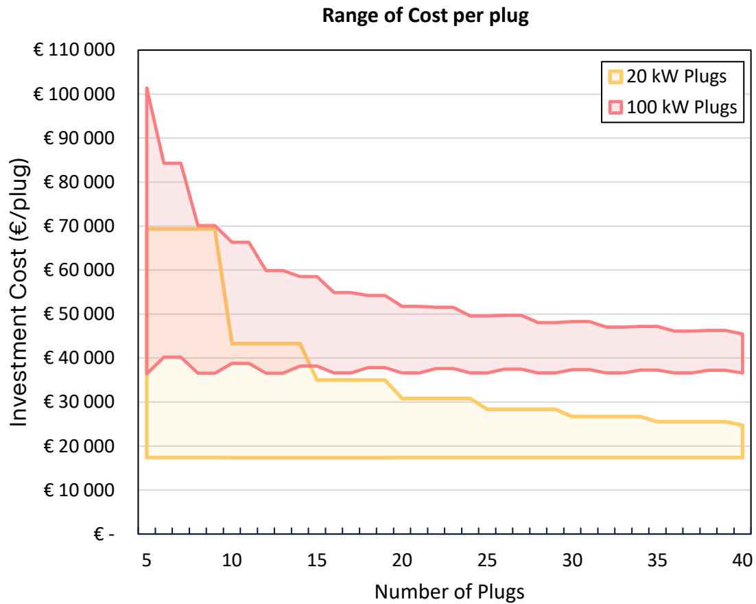
Figure 6: Investment cost per plug as a function of deployment scale, for 20 kW and 100 kW chargers.
