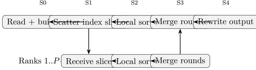
Figure 10: BSP like sketch of the distributed pipeline and its critical exchanges.
