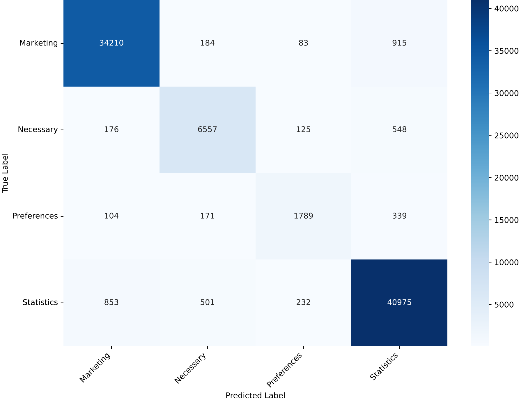
Confusion Matrix - KNN Test Accuracy: 95.18% Test F1 (macro): 89.62
