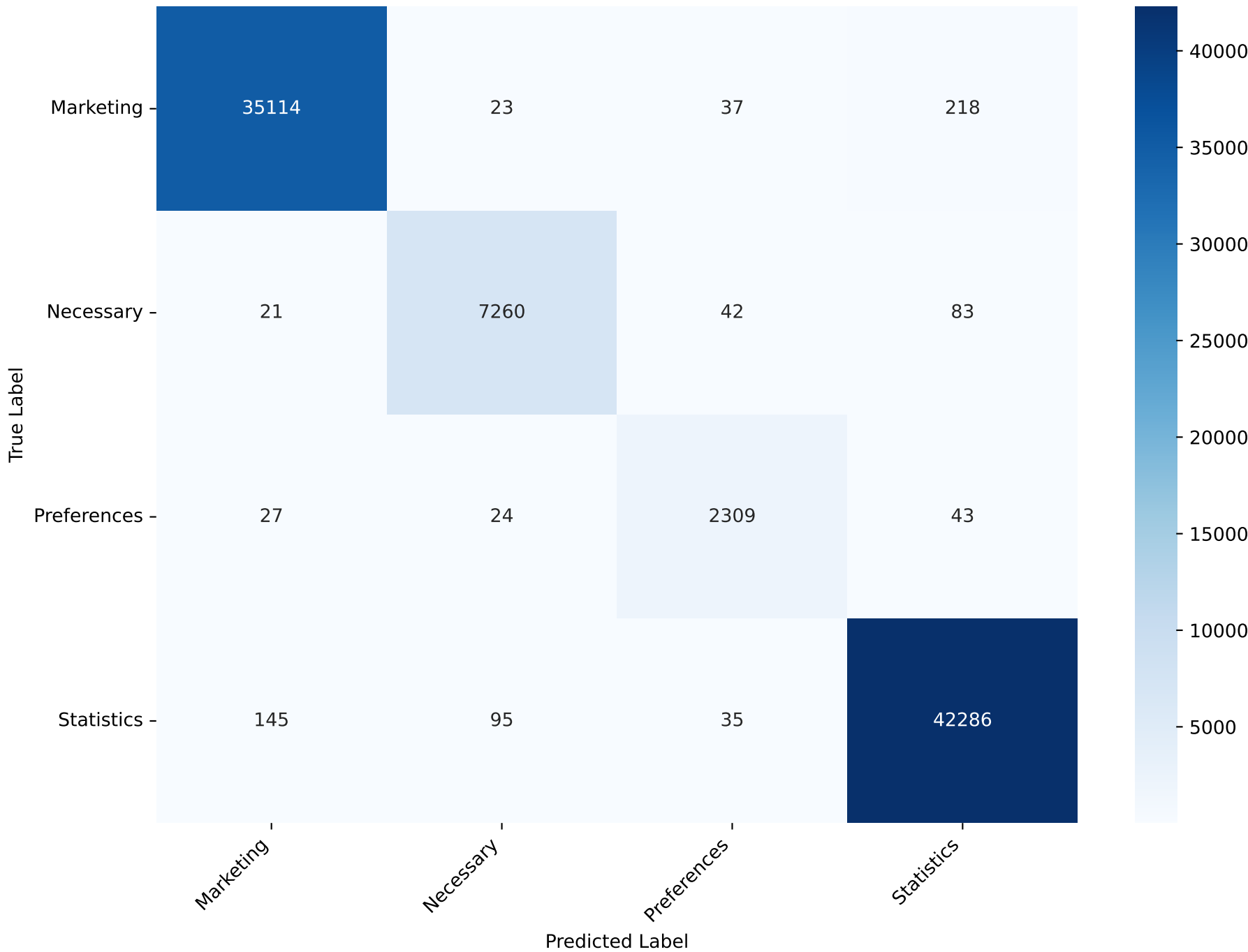
Confusion Matrix - MLP Test Accuracy: 99.10% Test F1 (macro): 98.09
