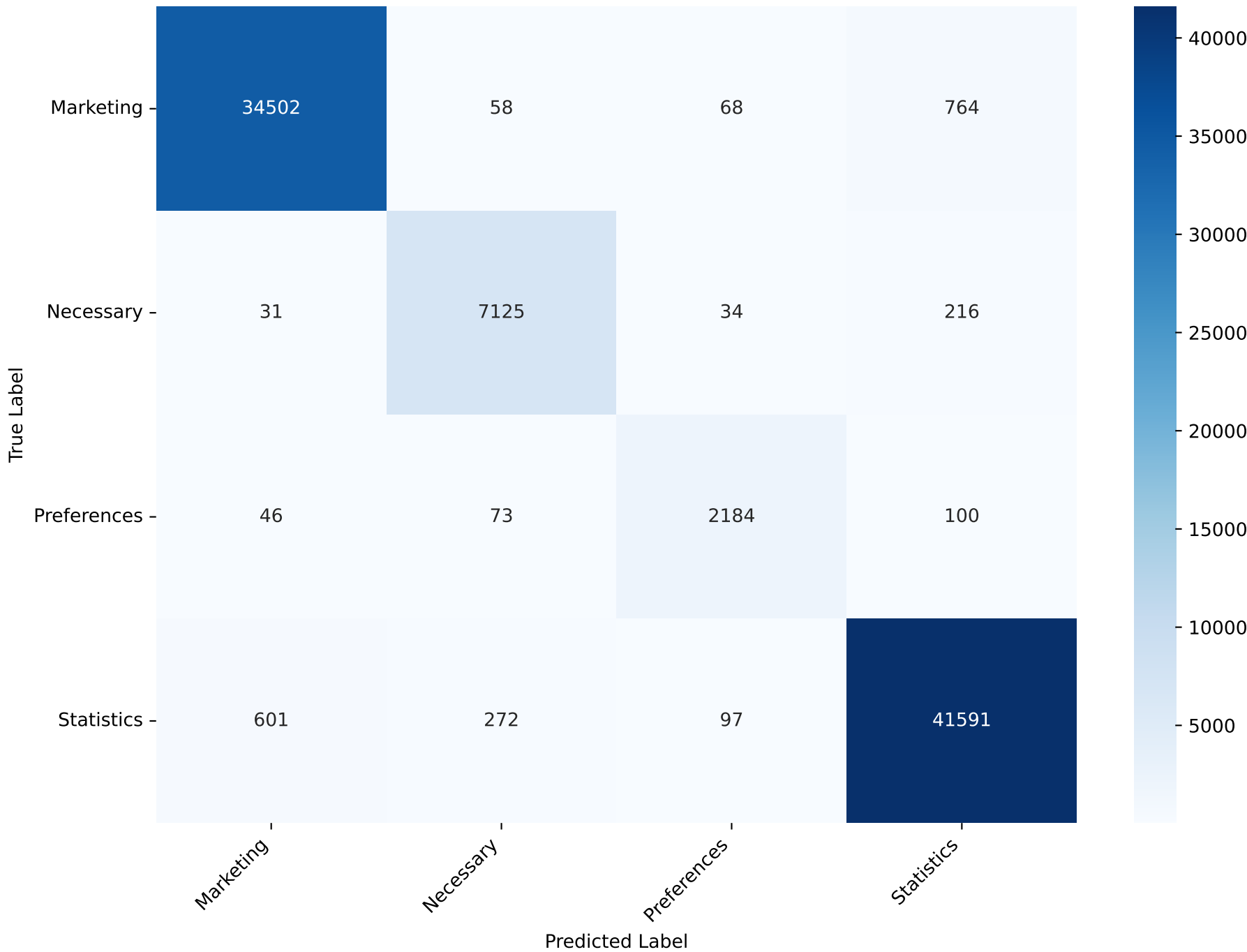
Confusion Matrix - PAC Test Accuracy: 97.31% Test F1 (macro): 95.51
