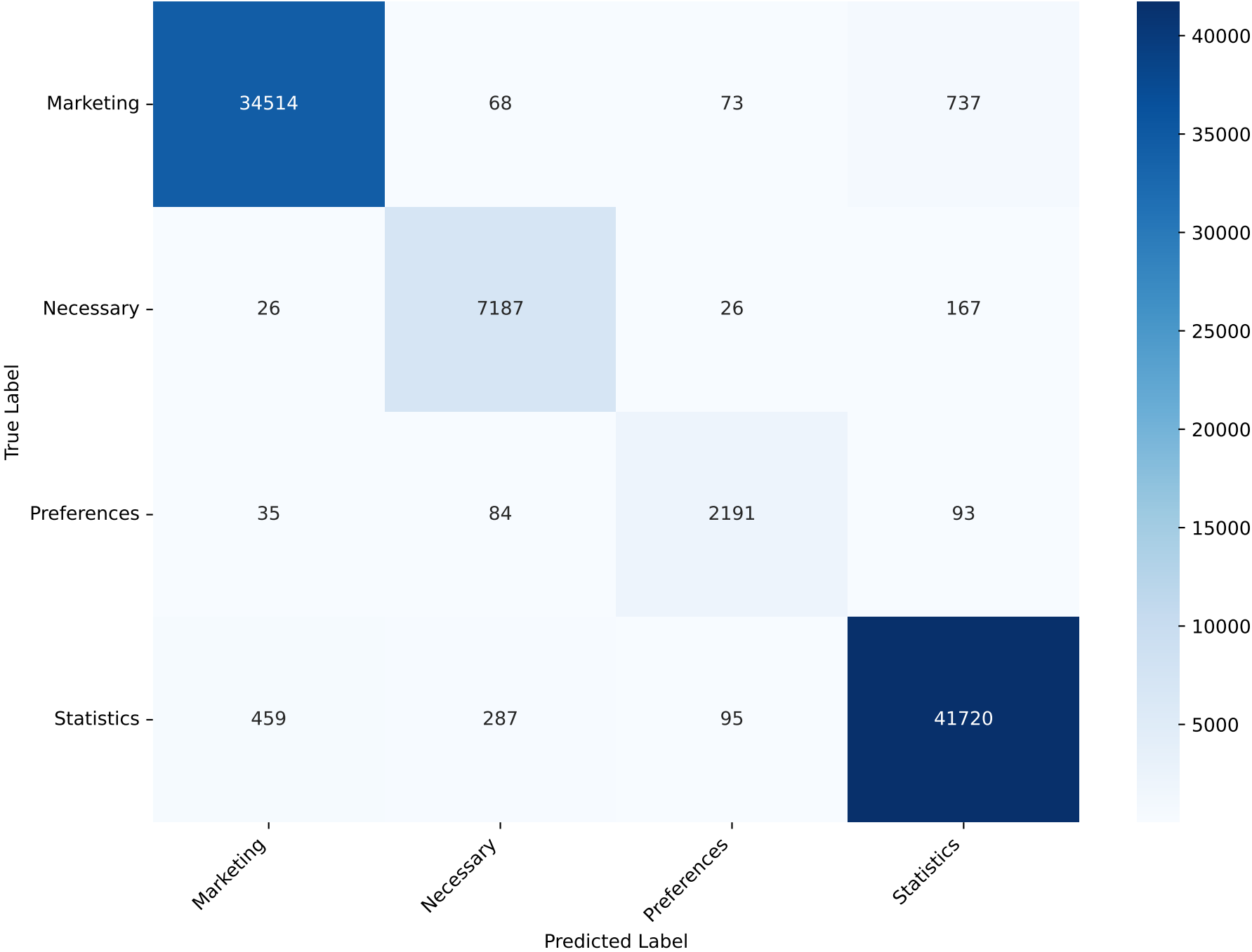
Confusion Matrix - SGD Test Accuracy: 97.55% Test F1 (macro): 95.75
