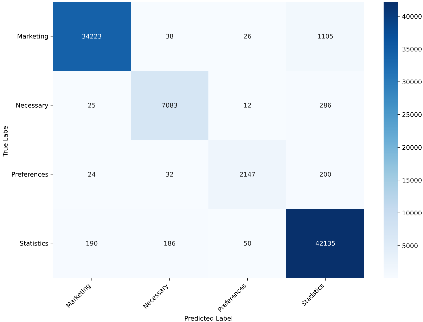
Confusion Matrix - XGBoost Test Accuracy: 97.52% Test F1 (macro): 96.08
