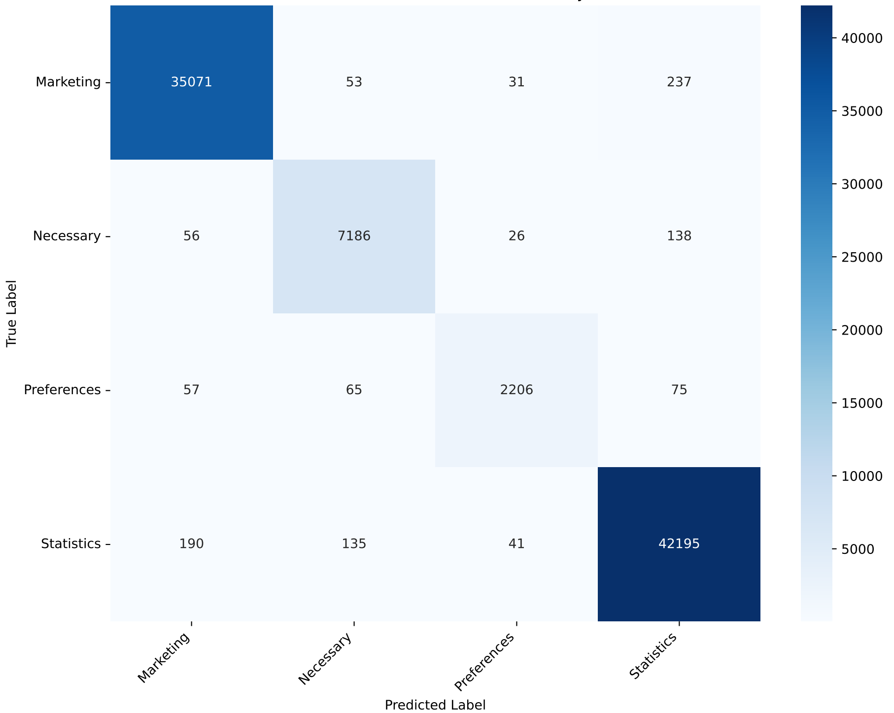
Confusion Matrix - MLP Classifier Test Accuracy: 98.74%
