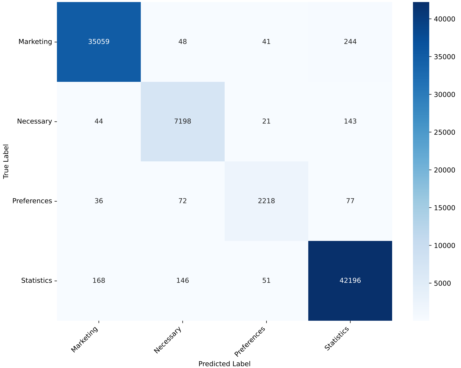
Confusion Matrix - MLP Classifier Test Accuracy: 98.76%
