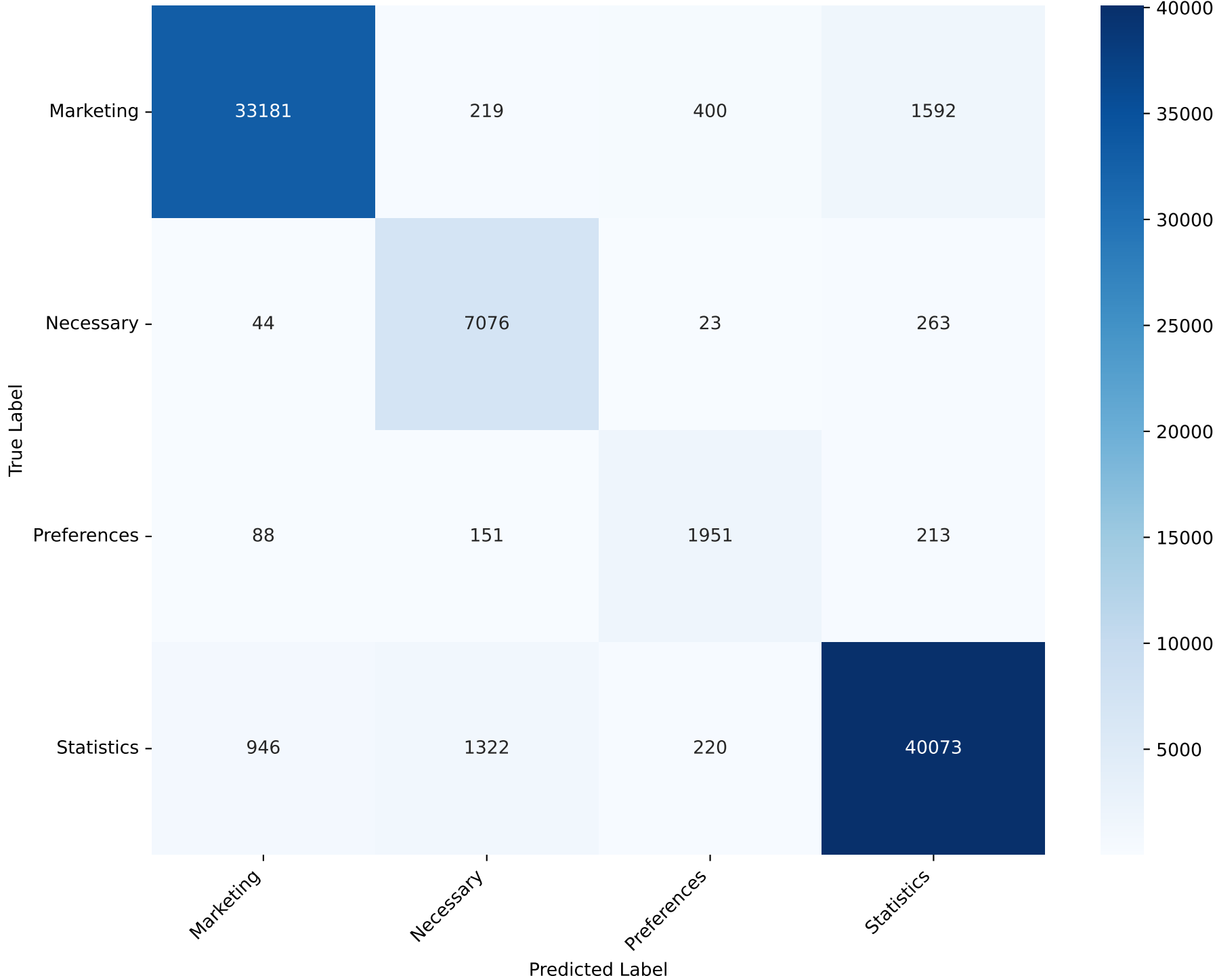
Confusion Matrix - Bernoulli Naive Bayes Test Accuracy: 93.75%
