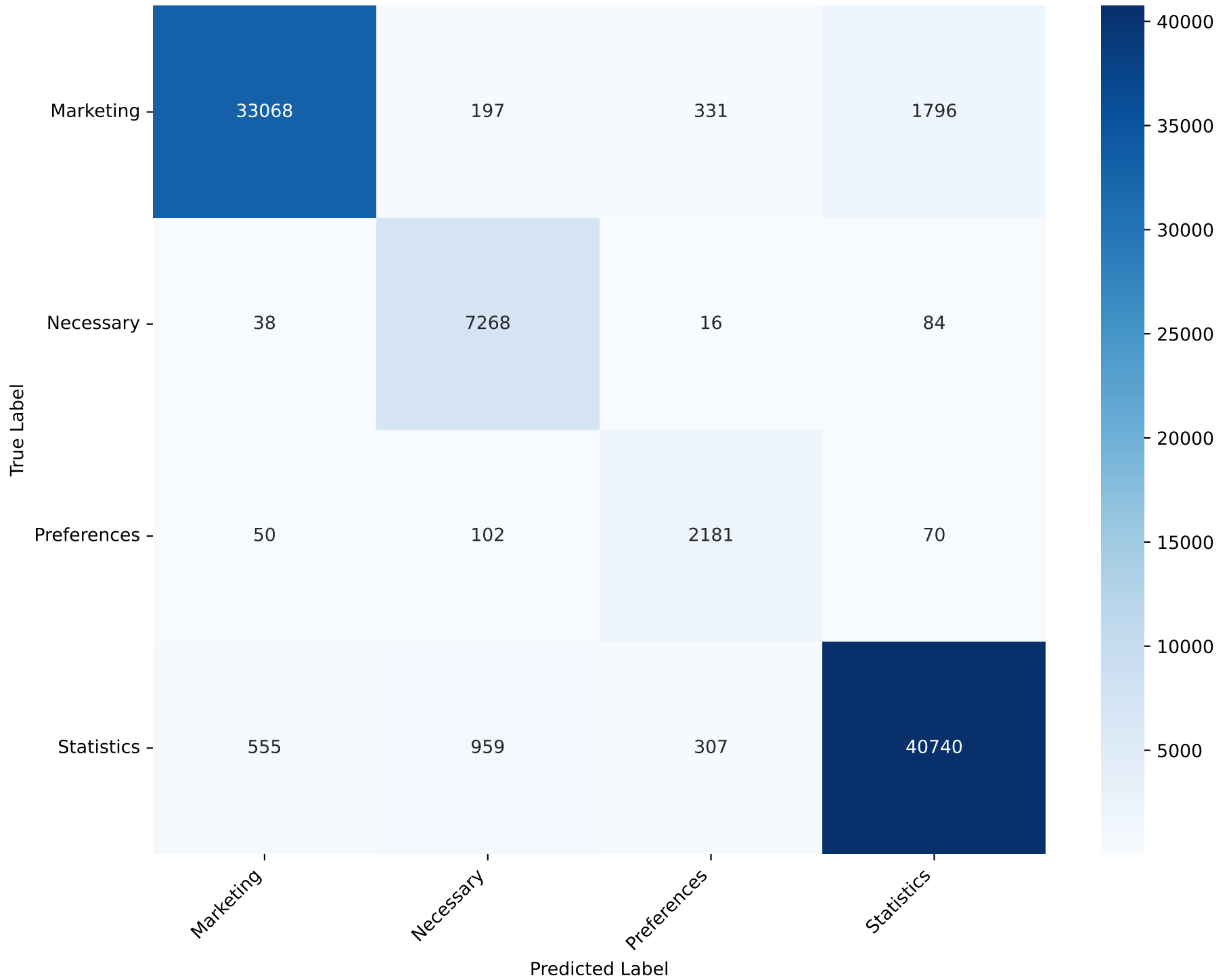
Confusion Matrix - Complement Naive Bayes Test Accuracy: 94.87%
