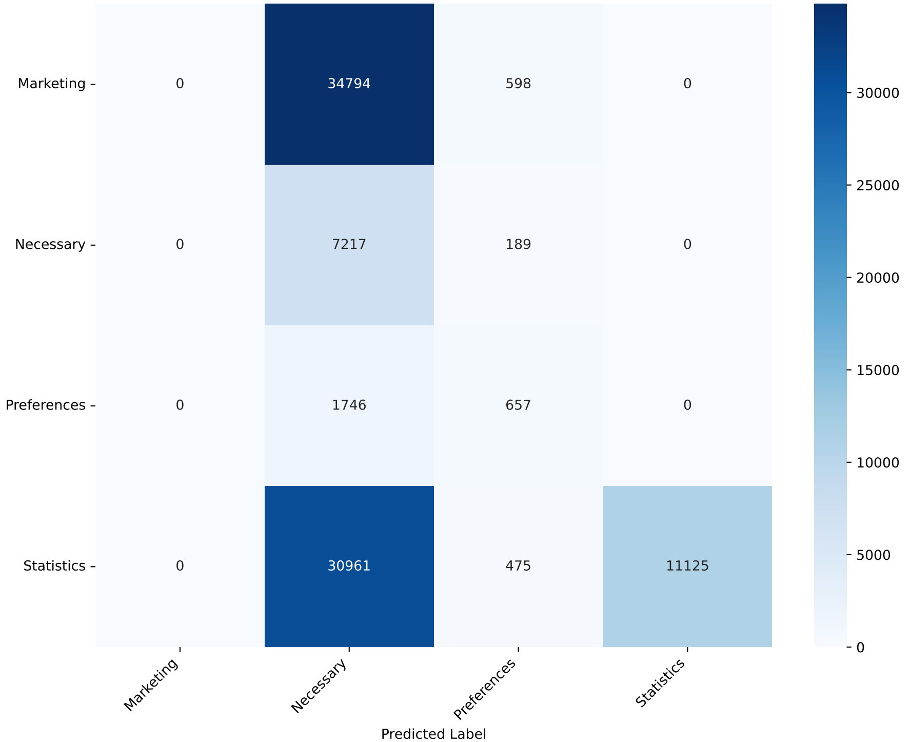
Confusion Matrix - Ada Boost Classifier Test Accuracy: 21.65%
