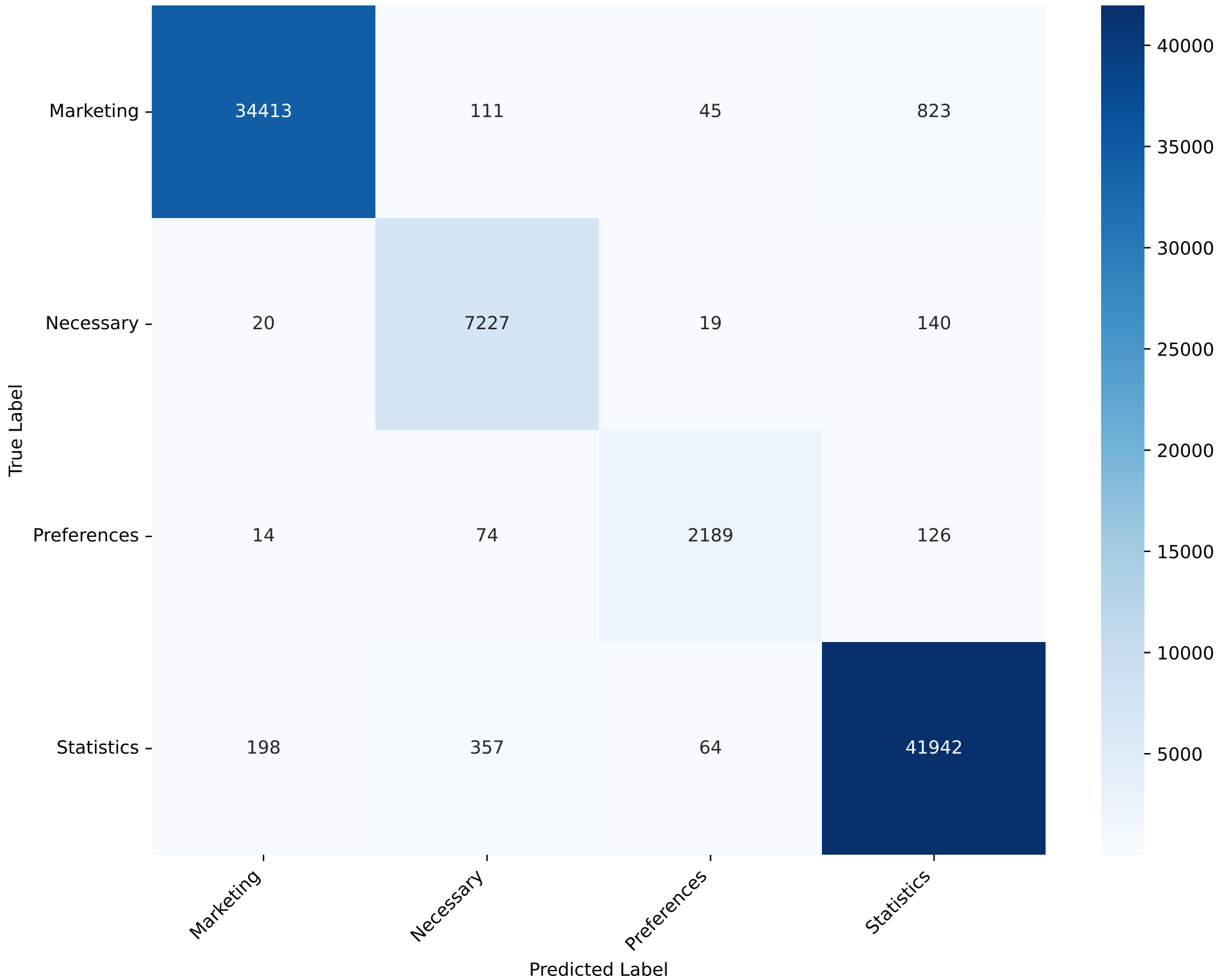
Confusion Matrix - CatBoost Classifier Test Accuracy: 97.73%
