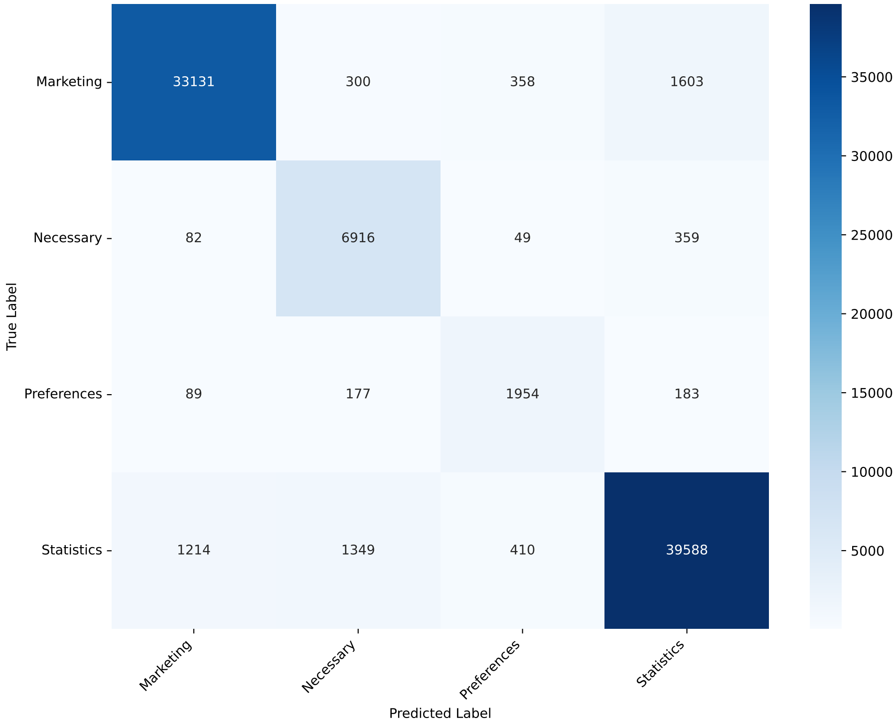
Confusion Matrix - Categorical Naive Bayes Test Accuracy: 92.97%
