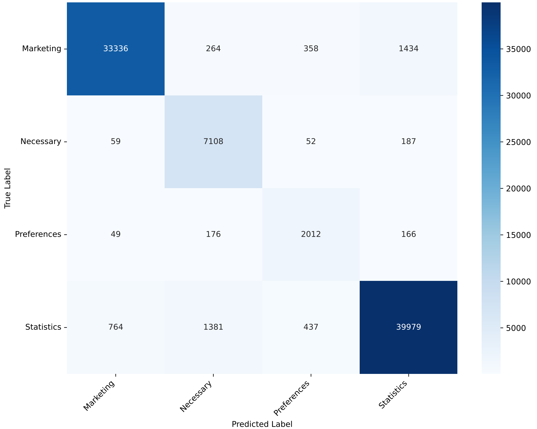
Confusion Matrix - Complement Naive Bayes Test Accuracy: 93.93%
