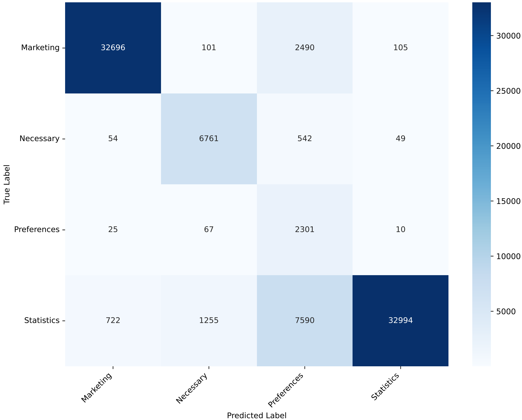
Confusion Matrix - Complement Naive Bayes + CountVectorizer Test Accuracy: 85.18%
