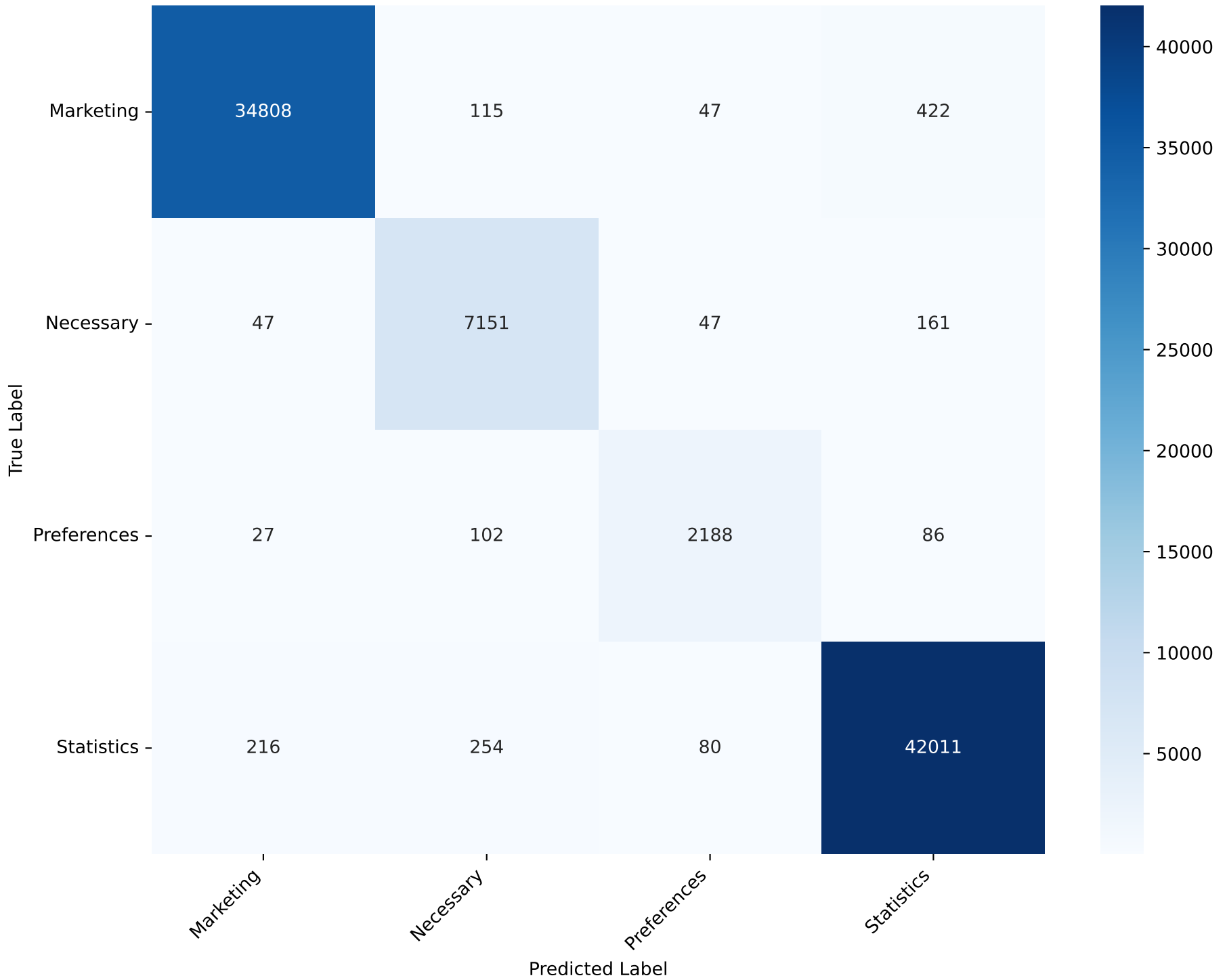
Confusion Matrix - Decision Tree Classifier Test Accuracy: 98.17%
