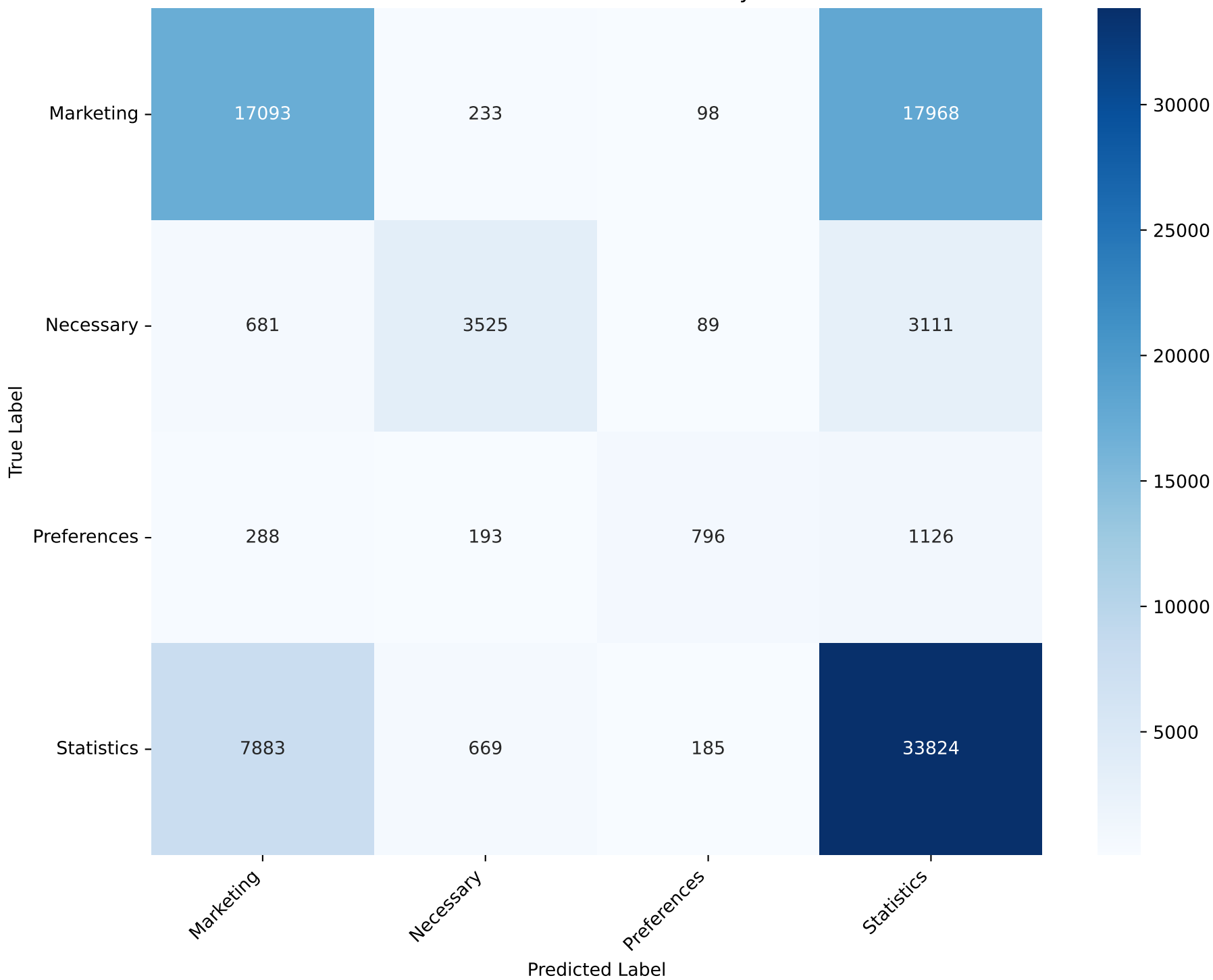
Confusion Matrix - KNN Test Accuracy: 62.94%
