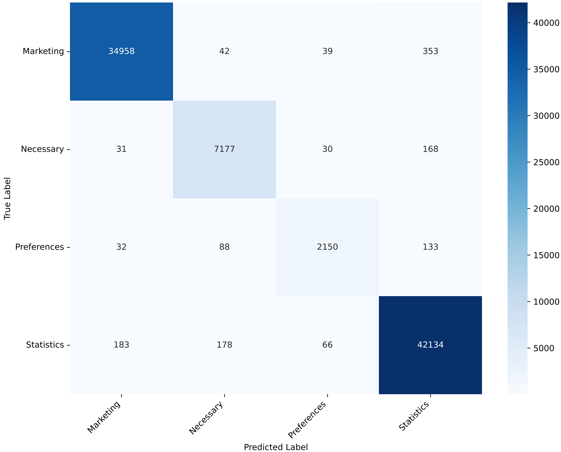
Confusion Matrix - LightGBM Classifier Test Accuracy: 98.47%
