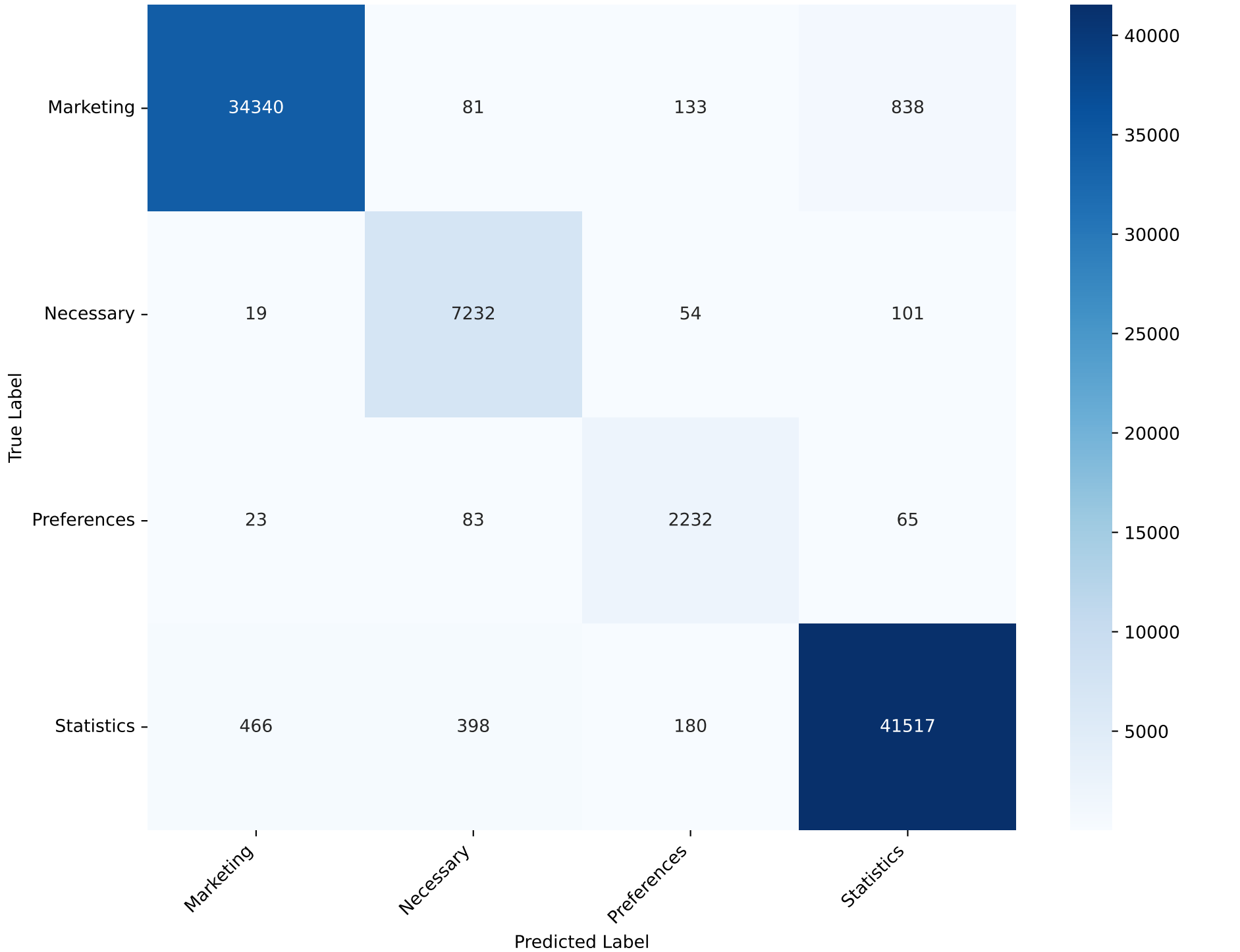
Confusion Matrix - LinearSVC Test Accuracy: 97.22%
