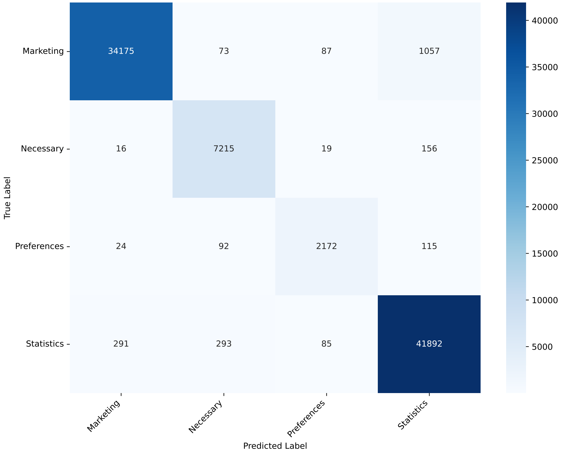
Confusion Matrix - LinearSVC Manual Weights Test Accuracy: 97.37%
