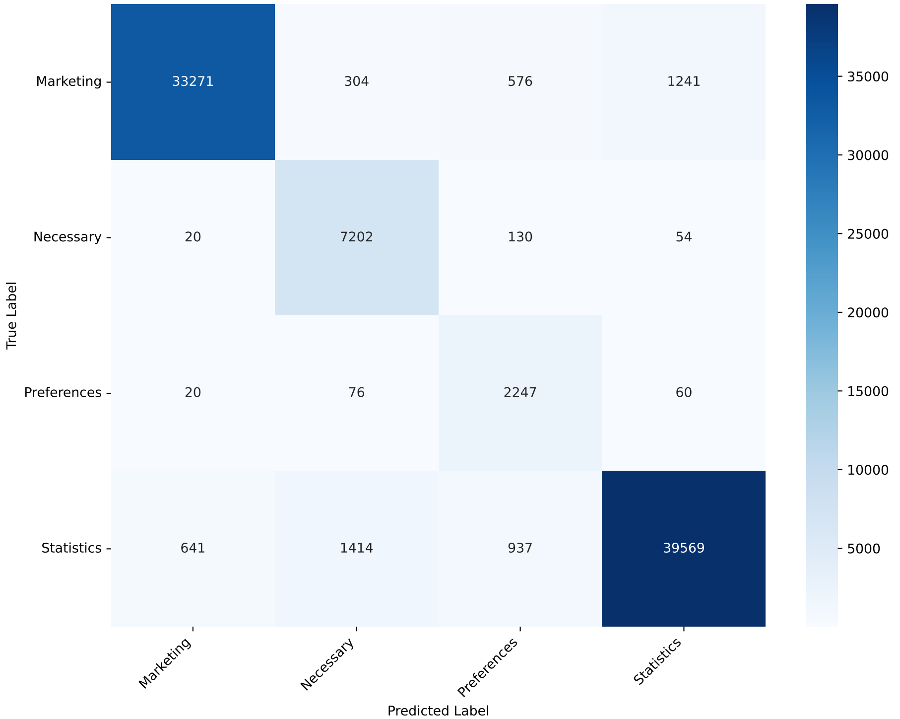
Confusion Matrix - Logistic Regression (Balanced) Test Accuracy: 93.76%
