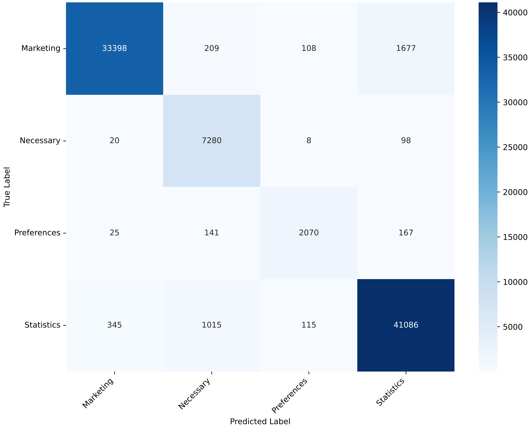
Confusion Matrix - Logistic Regression (Manual Weights) Test Accuracy: 95.52%
