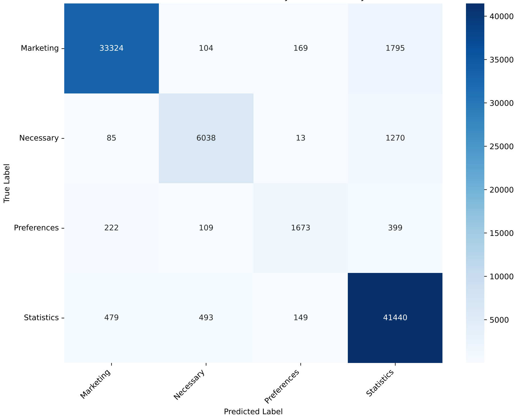
Confusion Matrix - Multinomial Naive Bayes Test Accuracy: 93.98%
