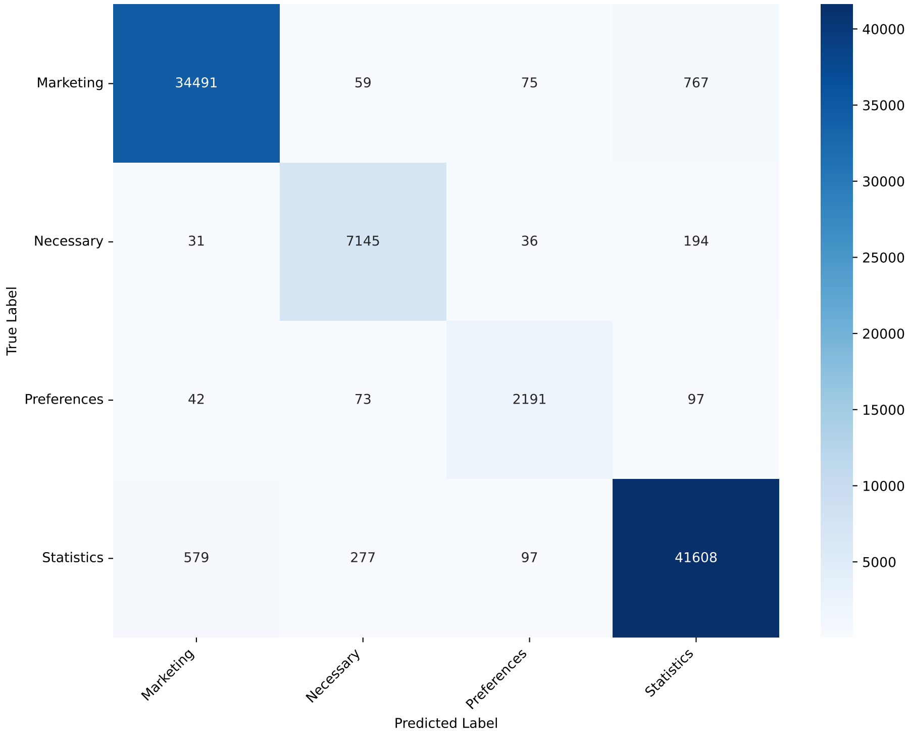
Confusion Matrix - Passive Aggressive Classifier Test Accuracy: 97.35%
