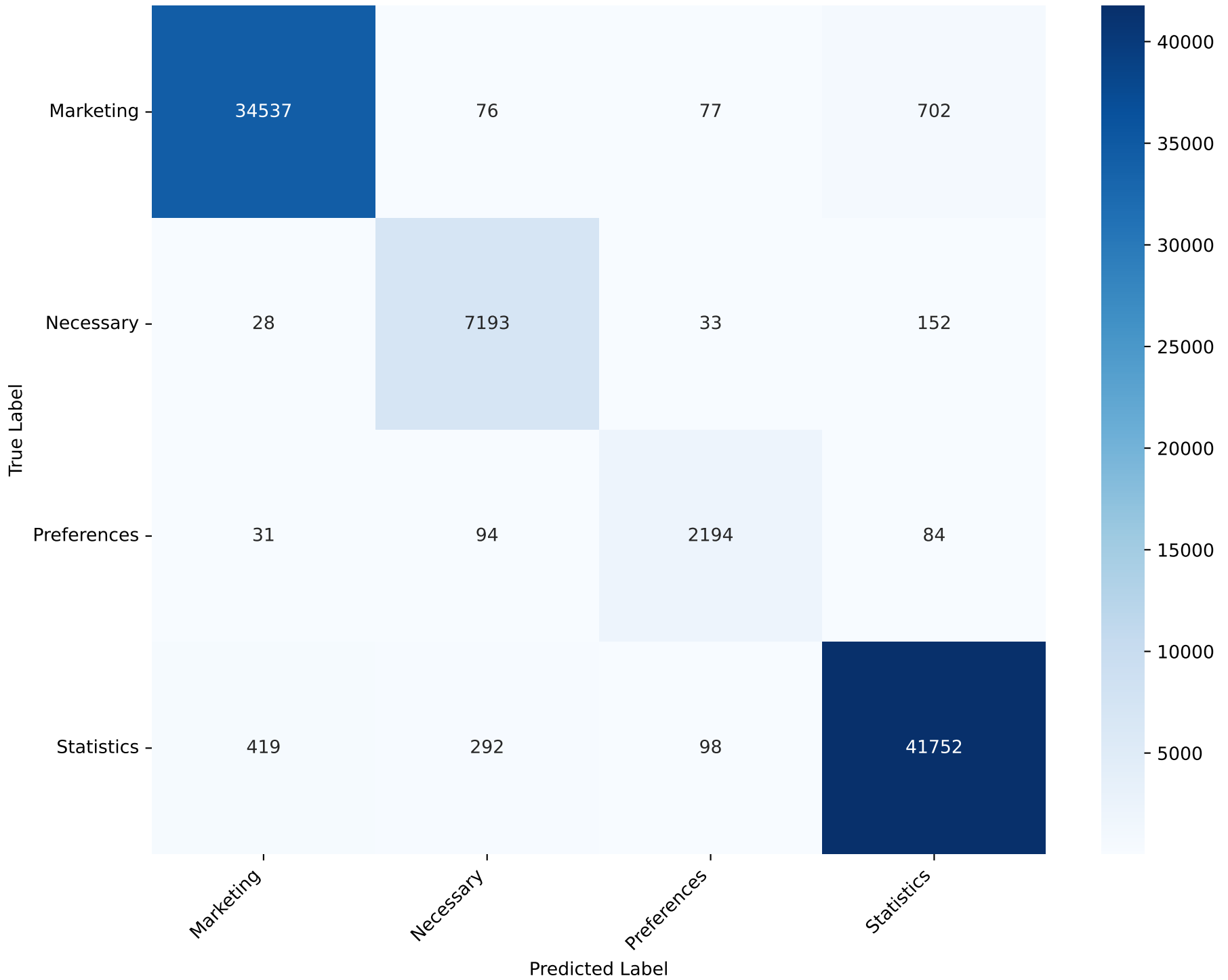
Confusion Matrix - SGD Classifier Test Accuracy: 97.62%
