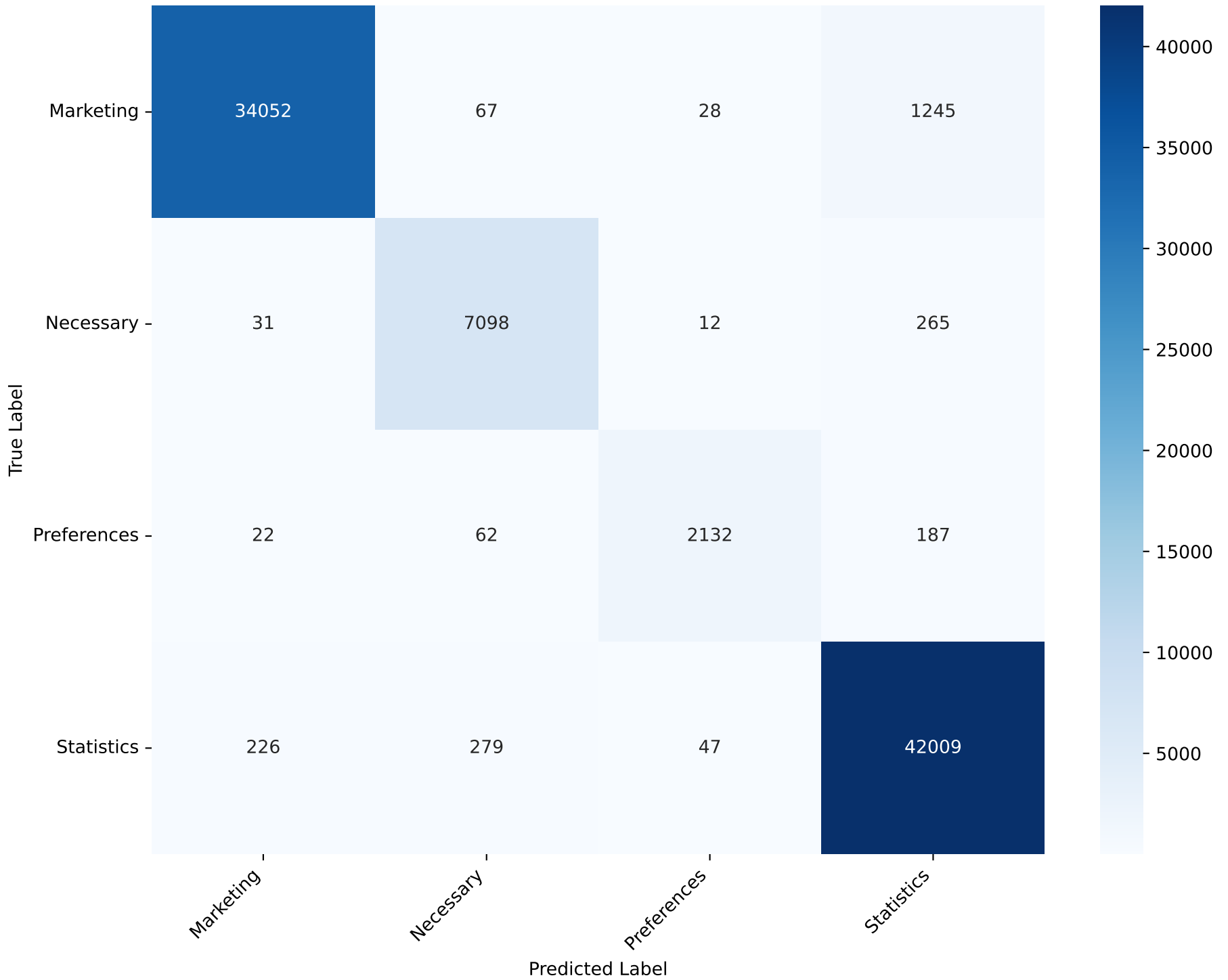
Confusion Matrix - XGBoost Classifier Test Accuracy: 97.18%
