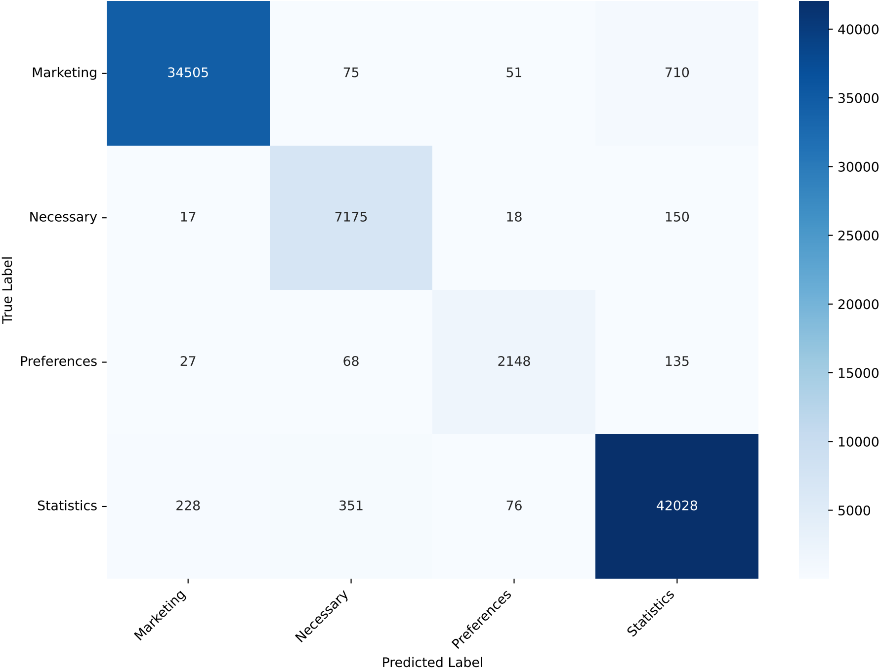
Confusion Matrix - CatBoost Test Accuracy: 97.83% Test F1 (macro): 95.99
