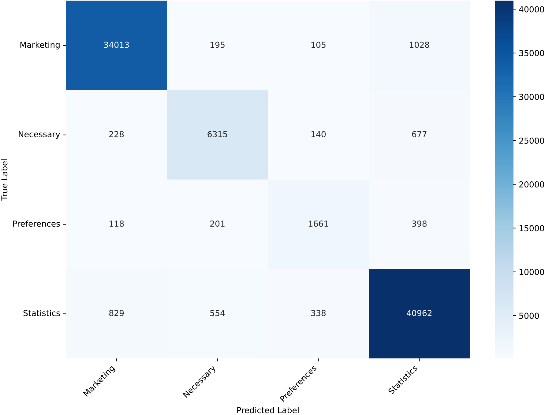
Confusion Matrix - KNN Test Accuracy: 94.52% Test F1 (macro): 87.56
