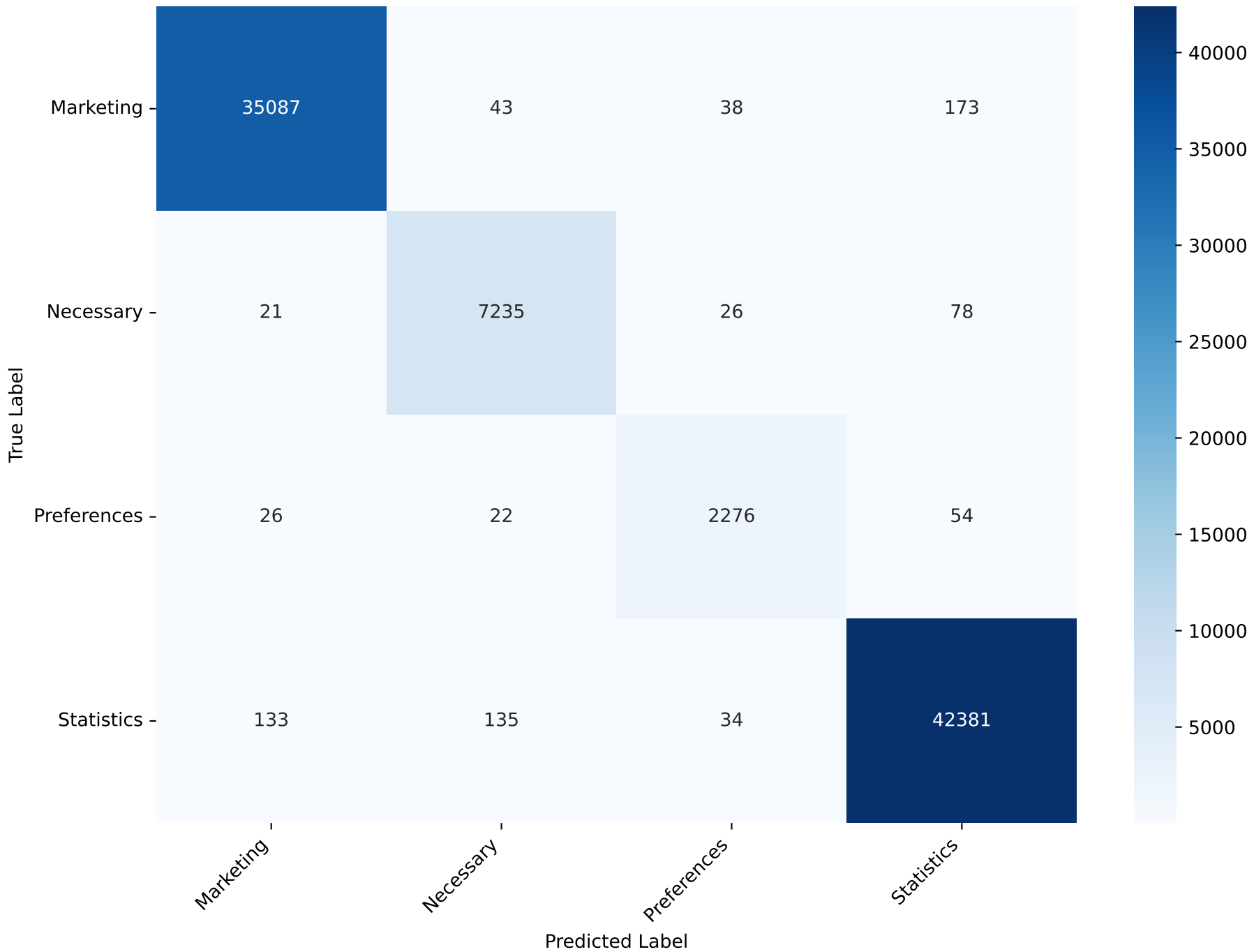
Confusion Matrix - MLP Test Accuracy: 99.11% Test F1 (macro): 98.07
