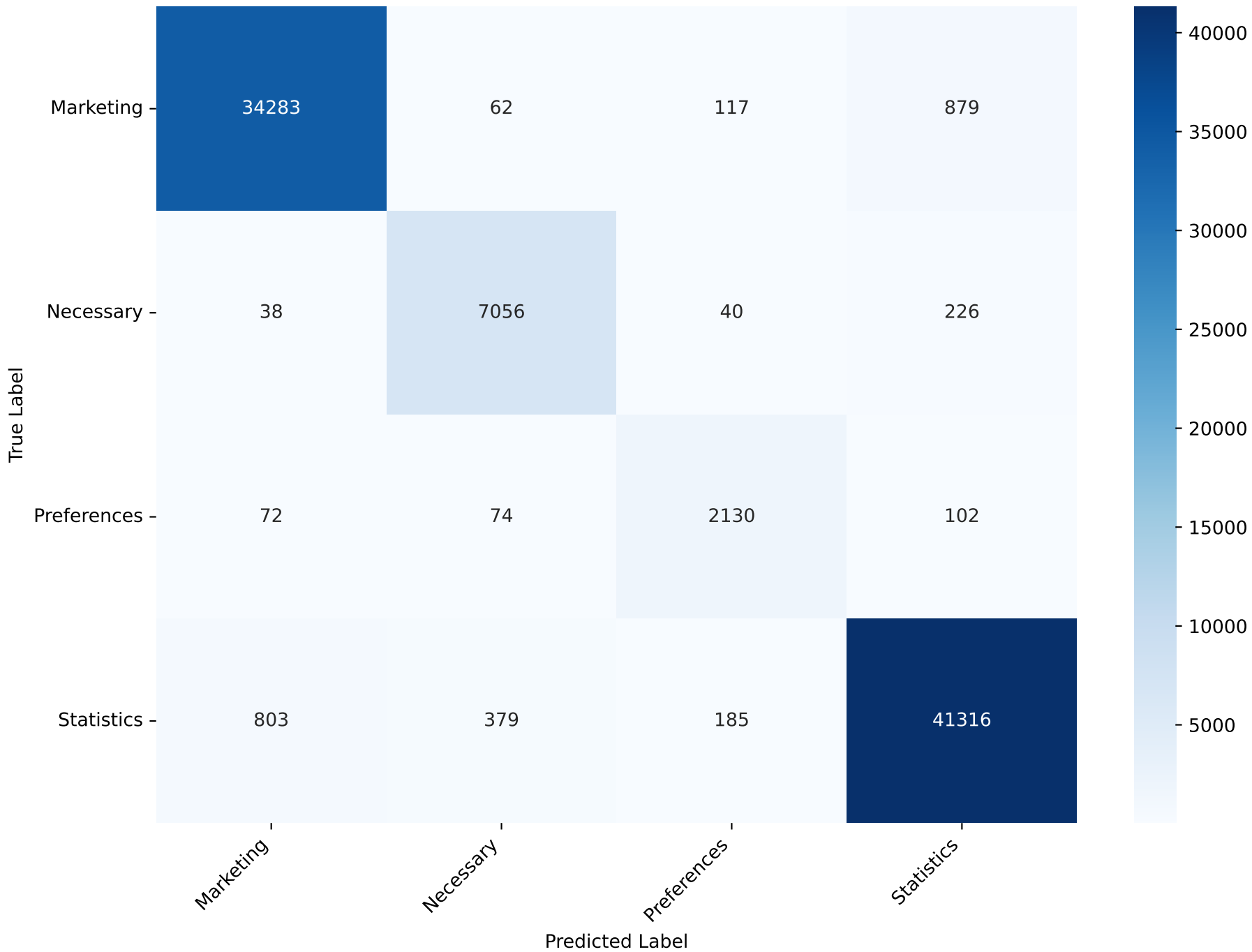
Confusion Matrix - PAC Test Accuracy: 96.61% Test F1 (macro): 94.13
