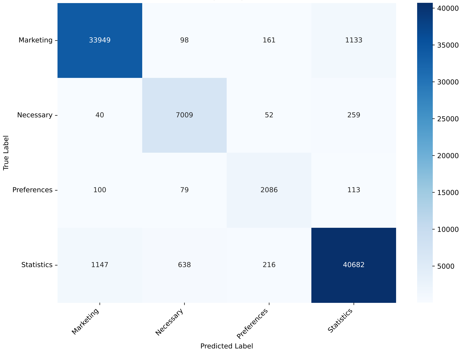
Confusion Matrix - Perceptron_MW
