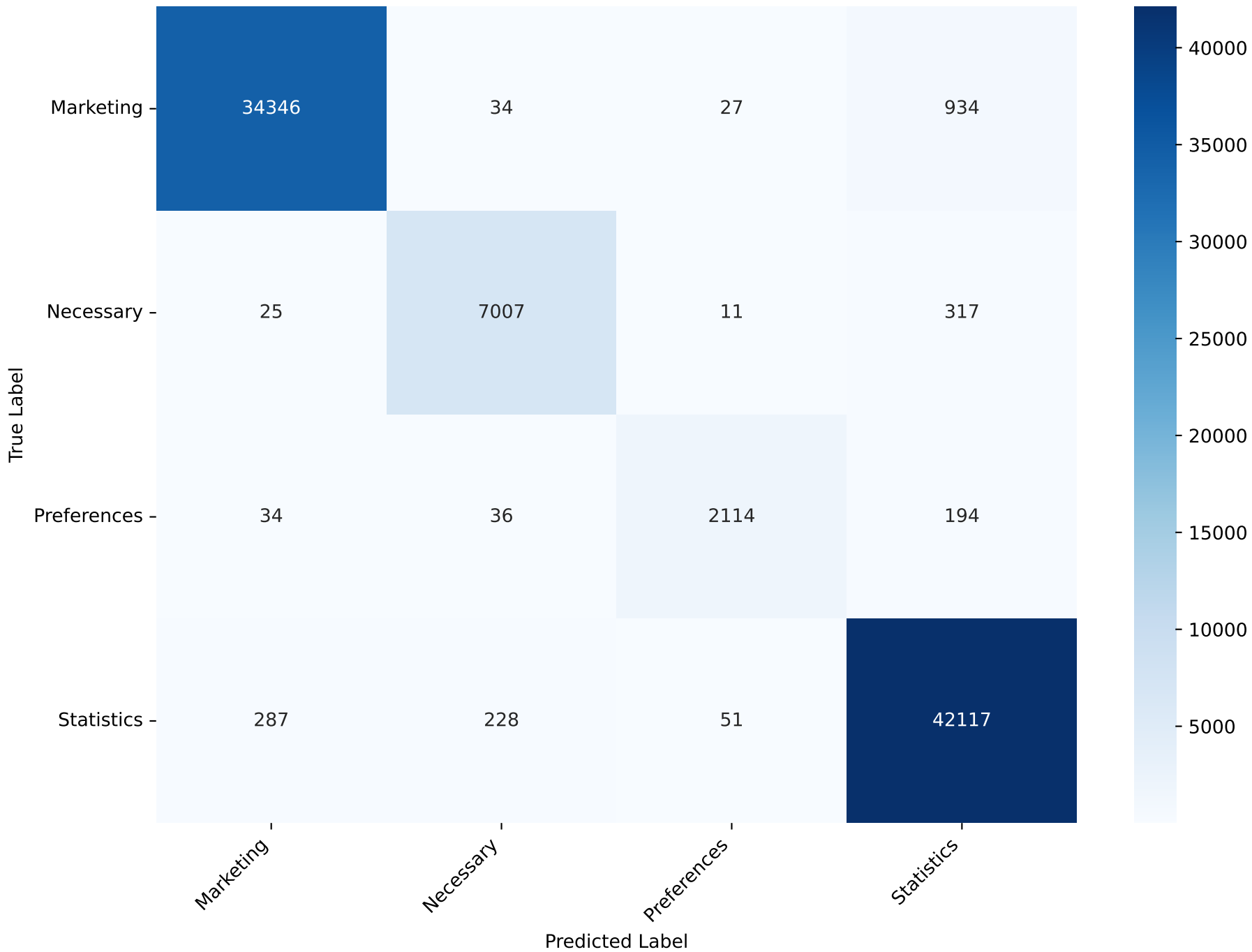
Confusion Matrix - XGBoost Test Accuracy: 97.52% Test F1 (macro): 95.90
