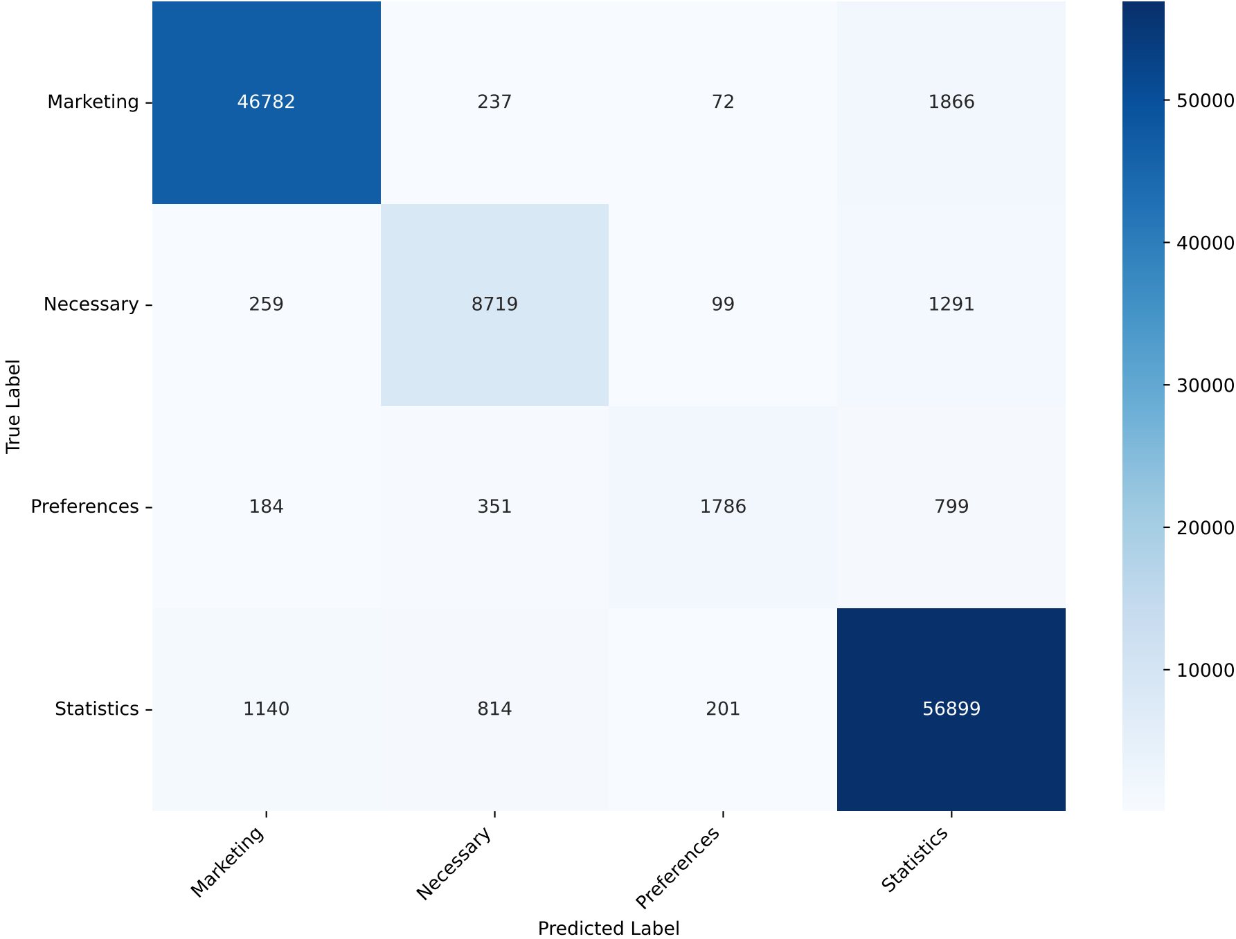
Confusion Matrix - AdaBoost Test Accuracy: 93.98% Test F1 (macro): 85.96
