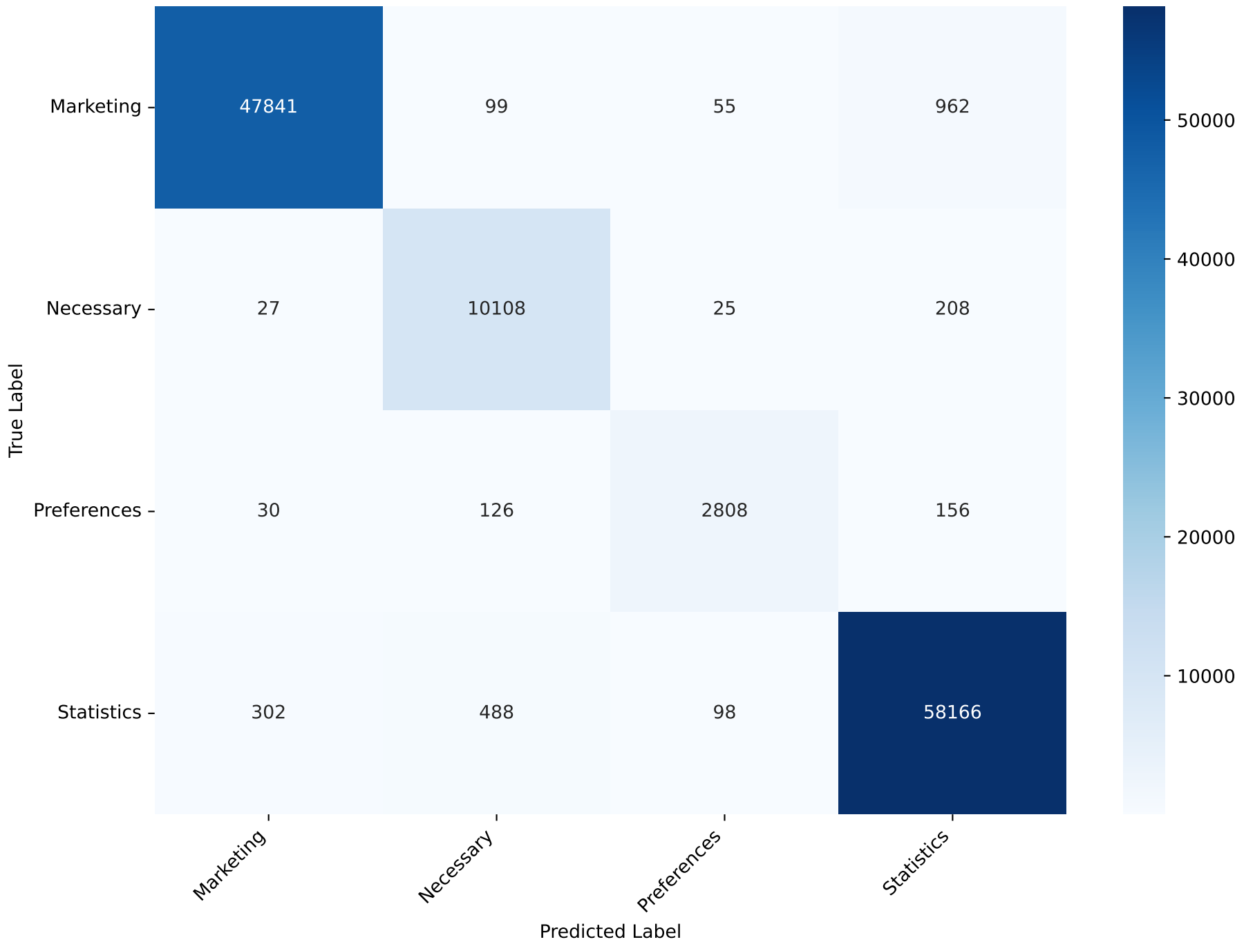
Confusion Matrix - CatBoost Test Accuracy: 97.88% Test F1 (macro): 96.00
