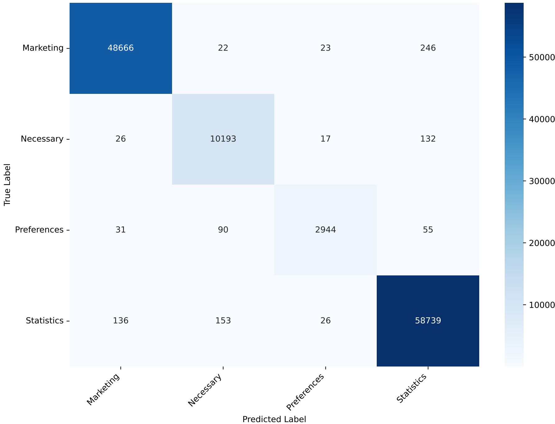
Confusion Matrix - MLP Test Accuracy: 99.21% Test F1 (macro): 98.20
