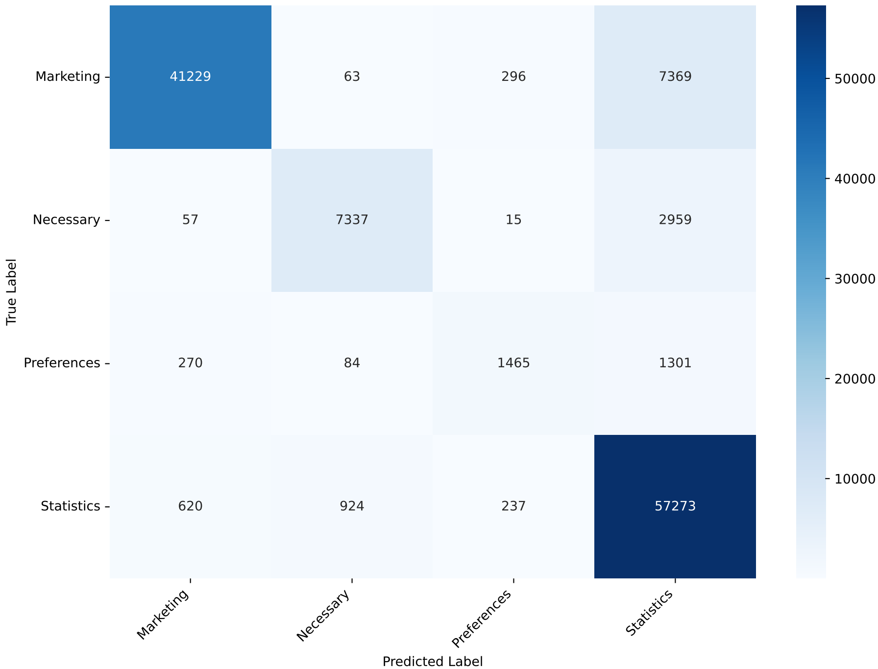
Confusion Matrix - NearestCentroid
