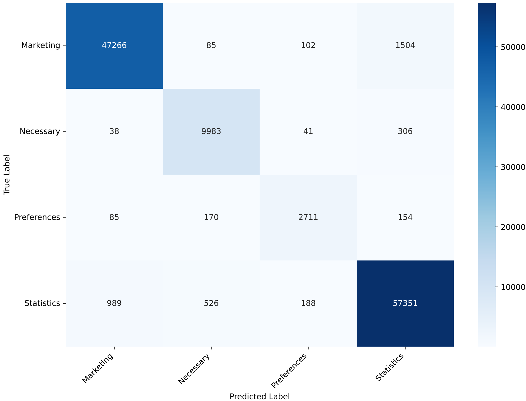
Confusion Matrix - PAC Test Accuracy: 96.55% Test F1 (macro): 94.12
