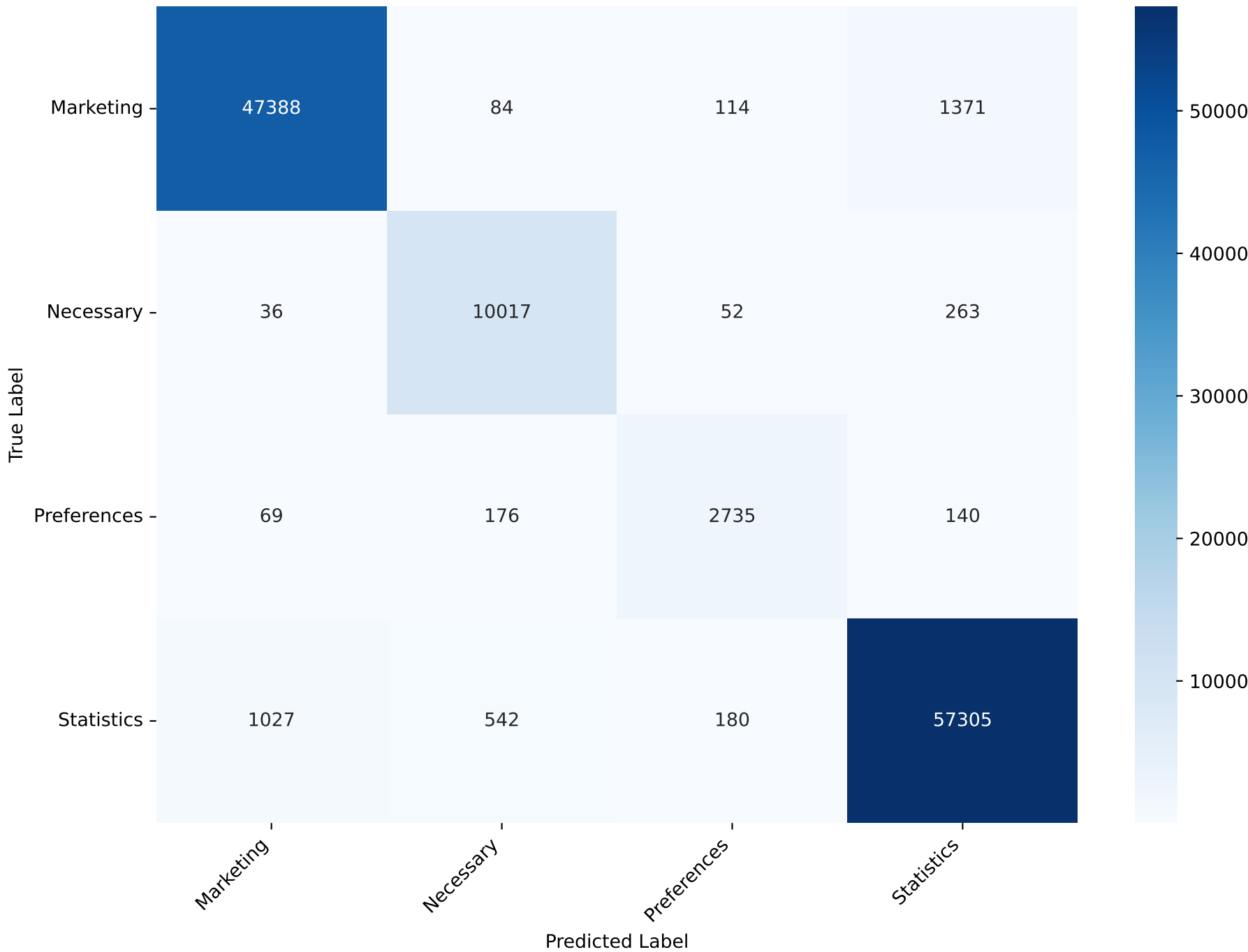
Confusion Matrix - SGD Test Accuracy: 96.66% Test F1 (macro): 94.25
