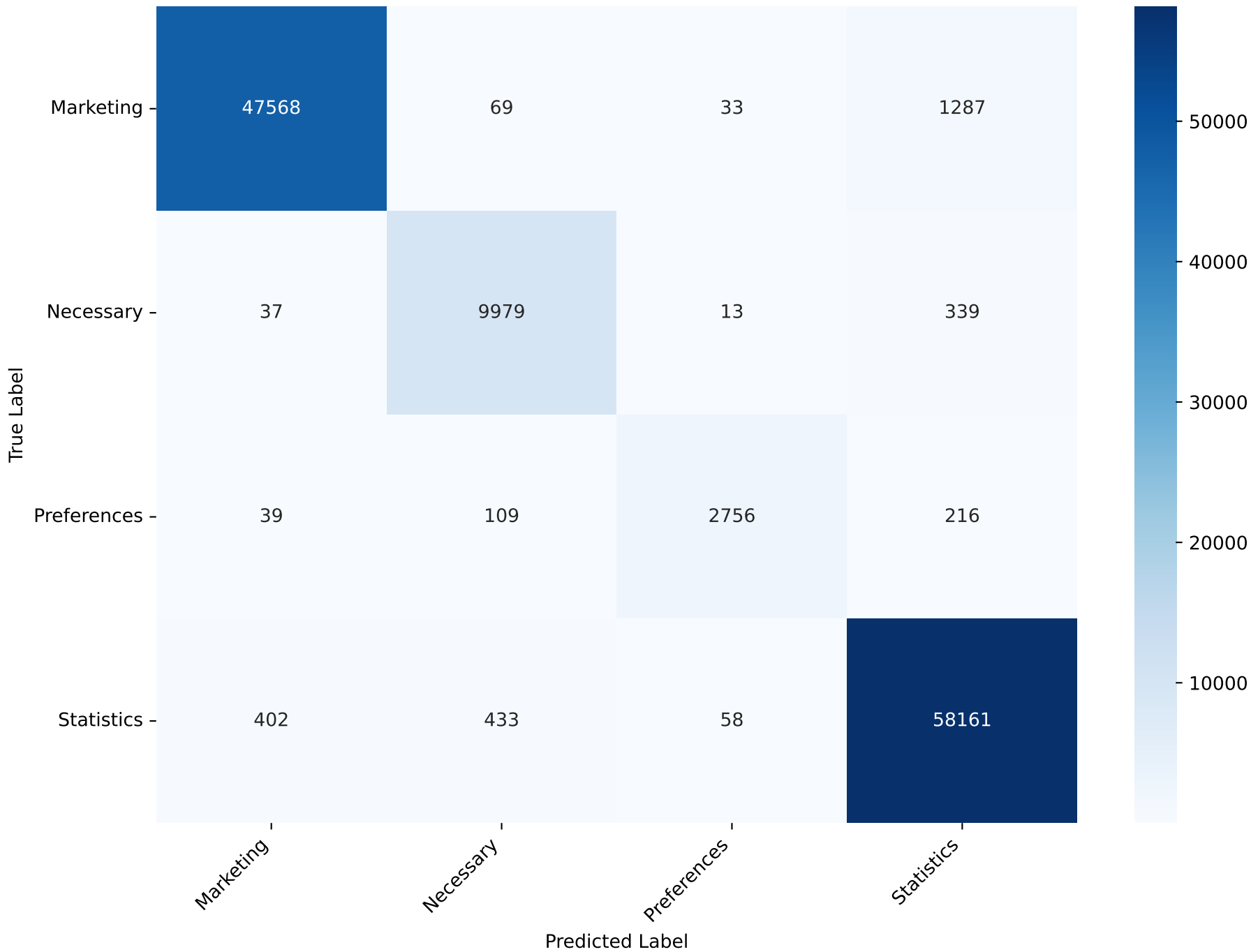
Confusion Matrix - XGBoost Test Accuracy: 97.50% Test F1 (macro): 95.80
