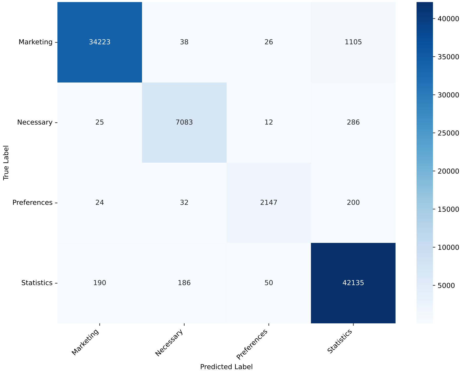
Confusion Matrix - XGBoost Classifier Test Accuracy: 97.52%
