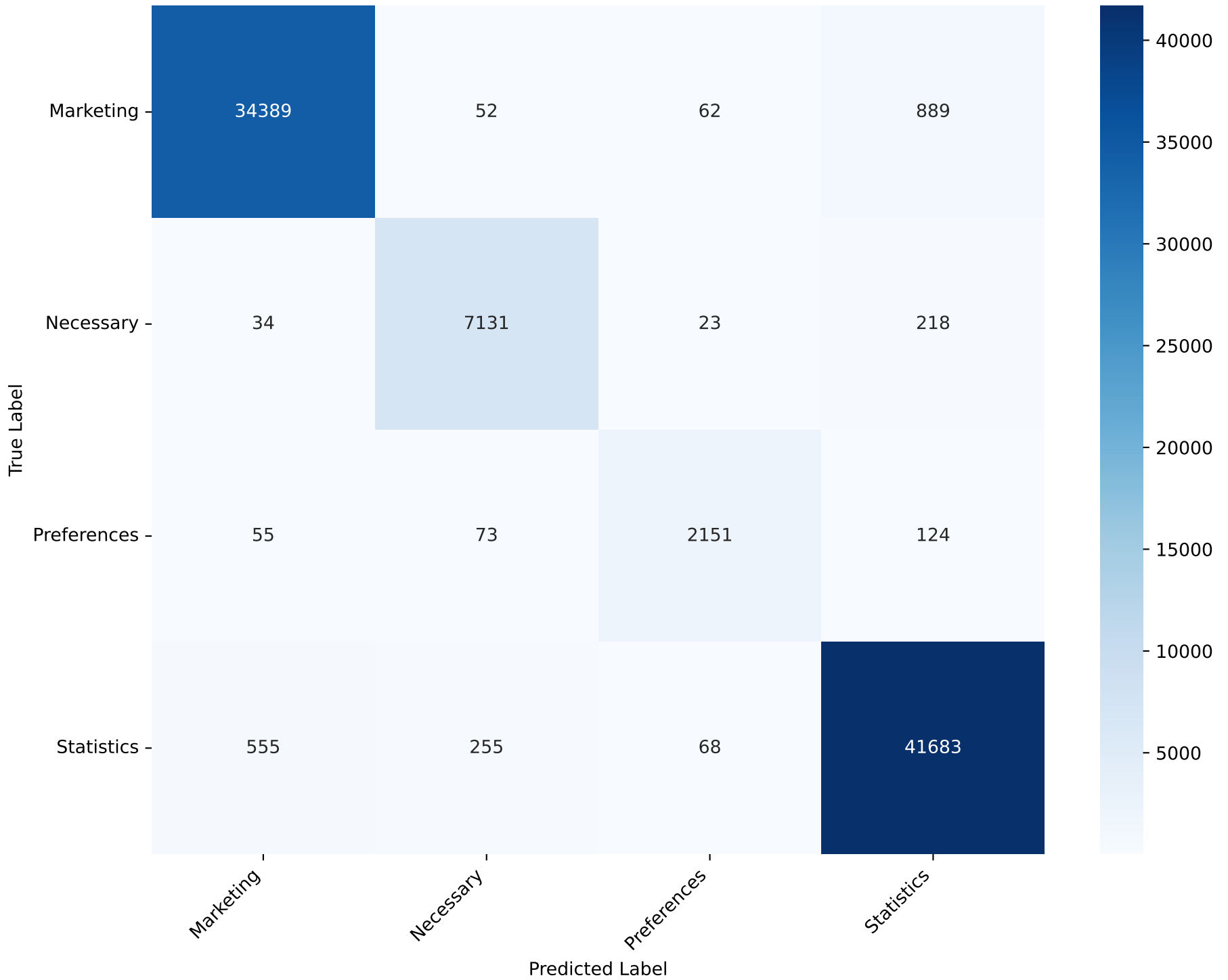
Confusion Matrix - Calibrated Classifier CV Test Accuracy: 97.26%
